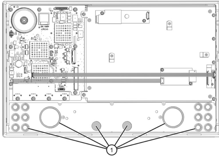
Figure 17 Lower Front Panel Overlay Replacement
