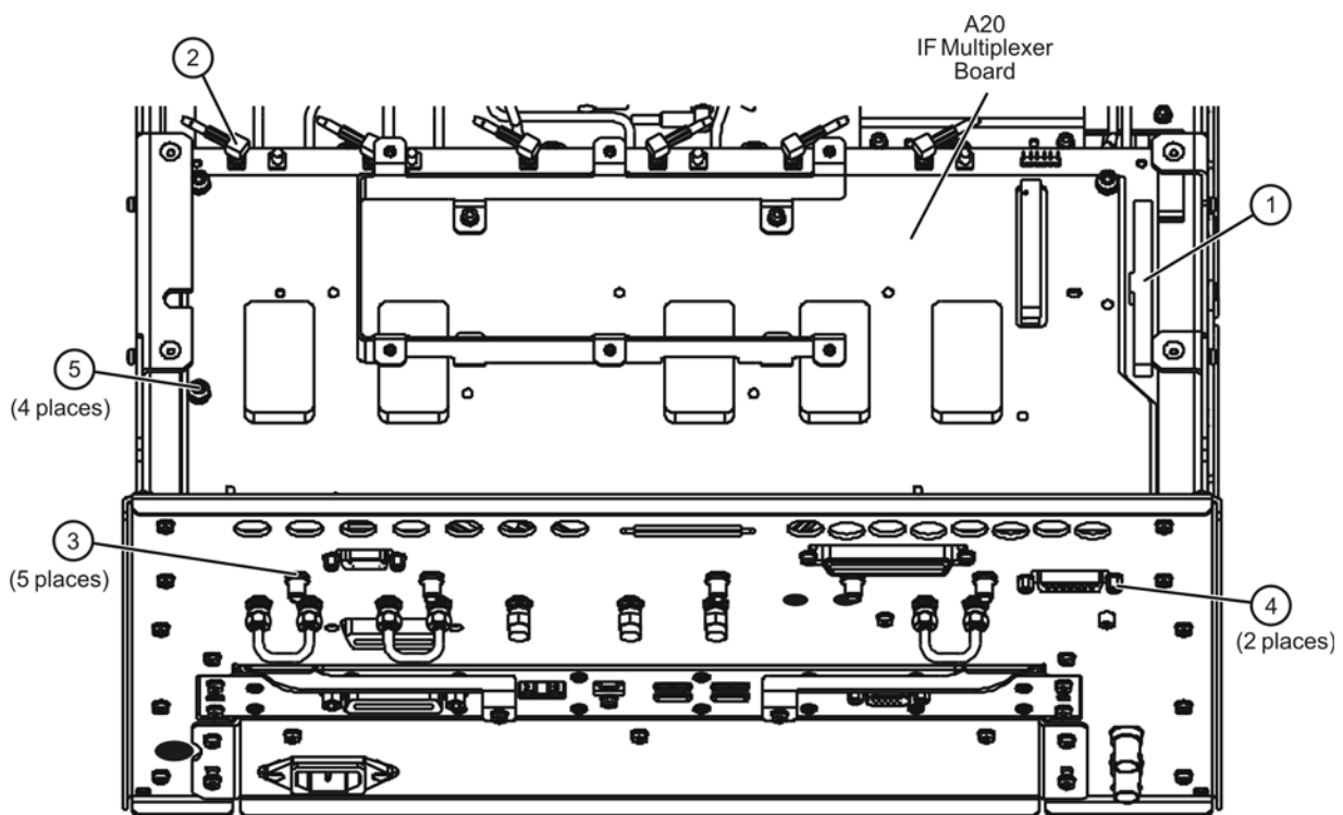
Figure 15 A20 IF Multiplexer Board Reinstallation
